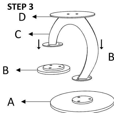
PLACE THE TOP OVER METAL FRAME
