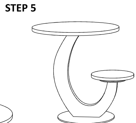
TIGHTEN THE BOTTOM WITH METAL FRAME BY SCREWS & ALLEN KEY ONE BY ONE
